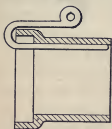
FIG. 19.—PIPE-LAYING Hook.
